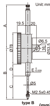
type B (mm)
