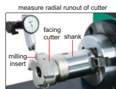
measure radial runout of cutter
