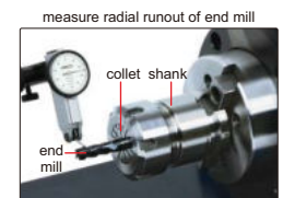
measure radial runout of end mill
