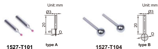
1527-T101 type A
