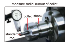
measure radial runout of collet
